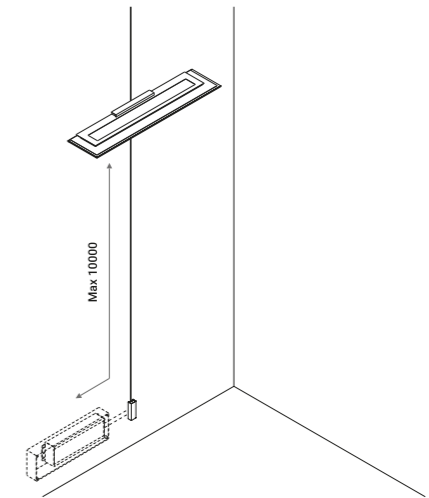
REFLEX - Installation with Endless and remote power supply kit
